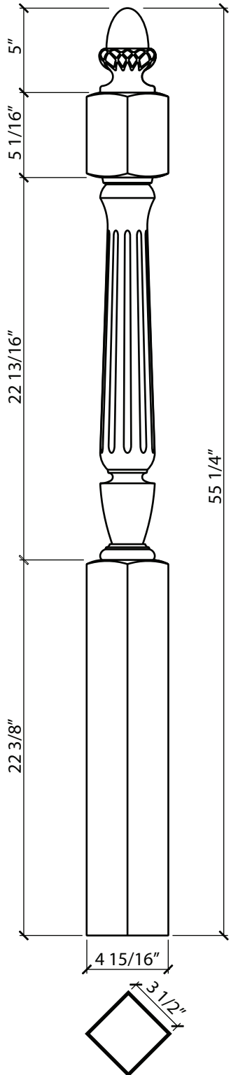
PNF503 3 1/2" x 55 1/4" COMBINATION NEWEL
