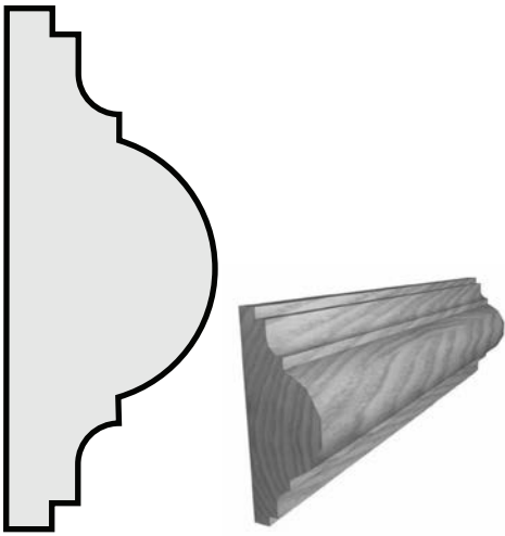
P32 1" x 2 1/2" ASTRAGAL
