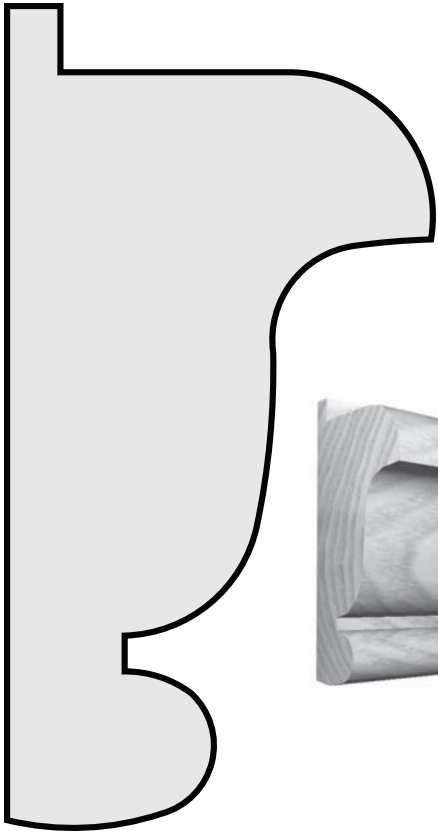
P124 2 1/4" x 4 5/16" PICTURE MOULD
