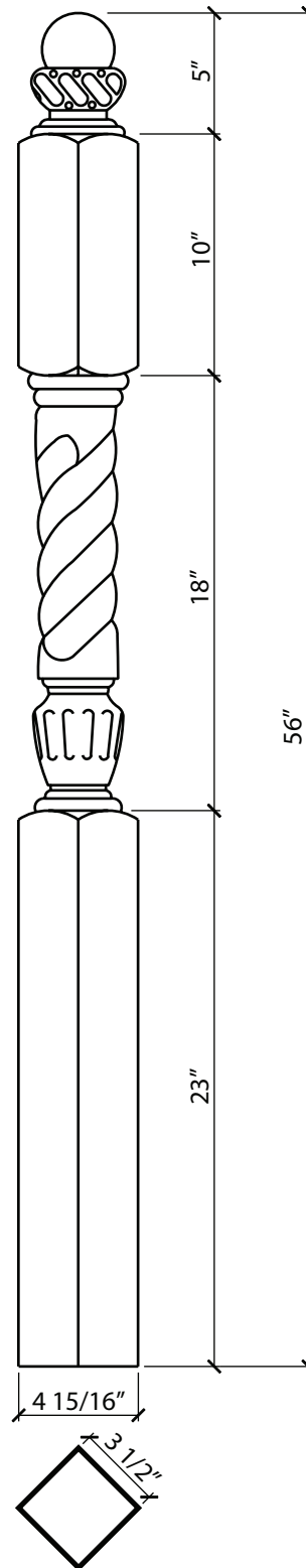
PNT702 3 1/2" x 56" LANDING NEWEL
