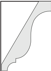
P186 1 3/4" x 9 7/16" CROWN/CORNICE
