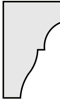
P41 1 1/16" x 1 3/4" FRIEZE MOULD
