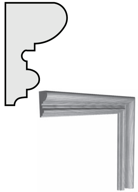
P84 1 1/16" x 1 3/4" PANEL MOULD
