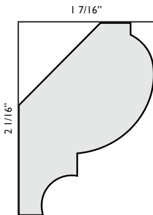
P266 1" x 2 1/16" COLUMN CAP/BASE
