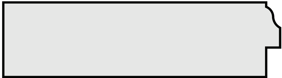
P227 1 3/8" x 5" SASH MOULD
