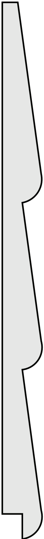
P207 1 1/16" x 9 1/4" STANDARD SIDING
