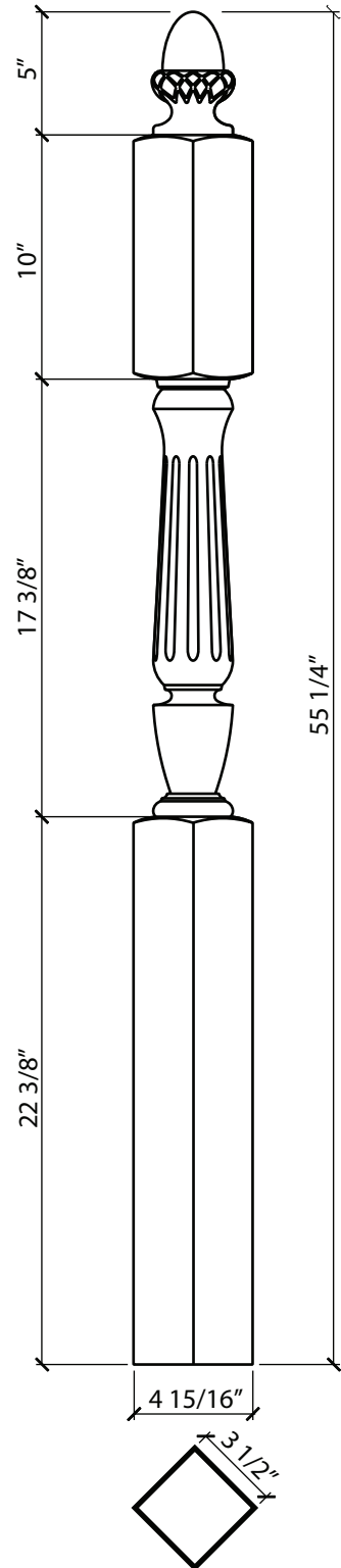
PNF504 3 1/2" x 55 1/4" LANDING NEWEL
