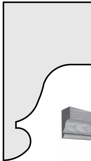
P86 3/4" x 1 15/16" PANEL MOULD
