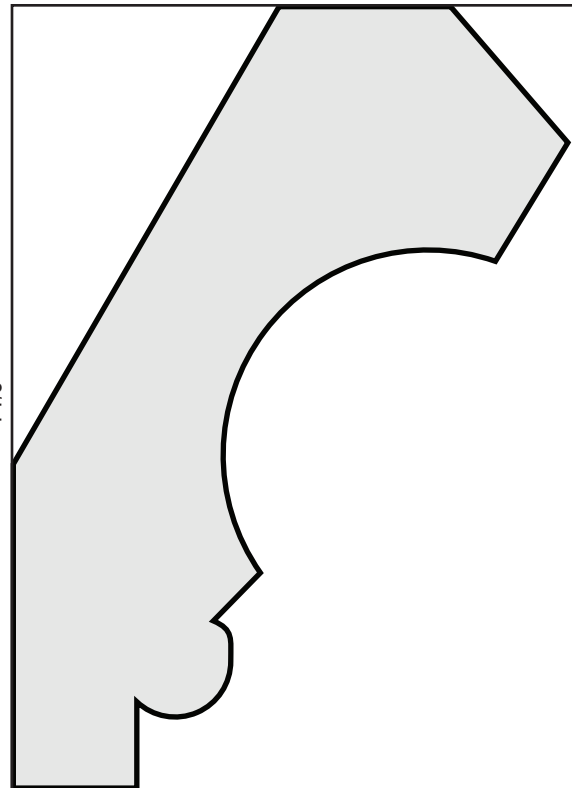
P184 1 5/8" x 4 11/16" CROWN/CORNICE
