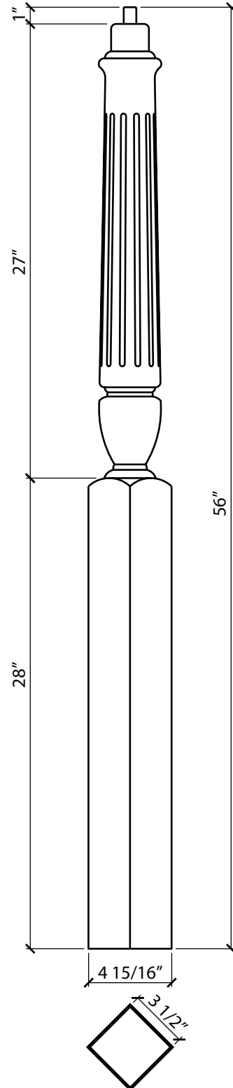
PNF502 3 1/2" x 56" LANDING NEWEL
